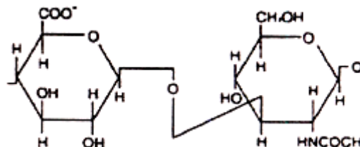
Structure of Hyaluronic acid
